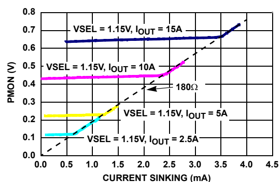
FIGURE 36. POWER MONITOR CURRENT SINKING CAPABILITY
