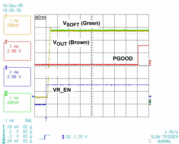
FIGURE 14. SOFT-START WAVEFORM SHOWING PGOOD
