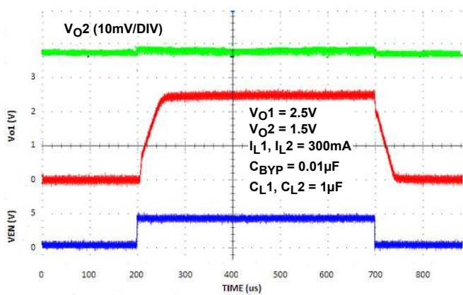
FIGURE 13. TURN-ON/TURN-OFF RESPONSE
