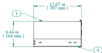
SIDE VIEW WITHOUT SHROUD
