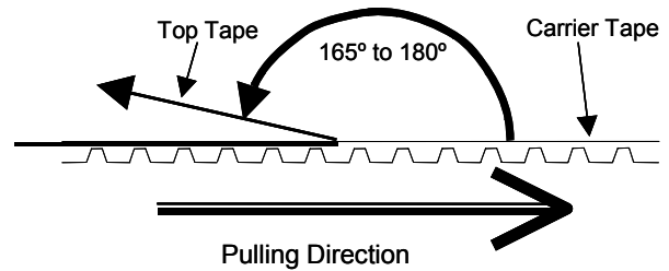
Fig.8 Peeling Strength
