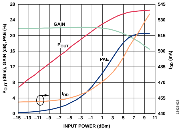
Figure 28. P_{OUT} , Gain, PAE, and I_{DD} vs. Input Power, RF = 73.5 GHz, Drain Current ( I_{DD} ) = 450 mA
