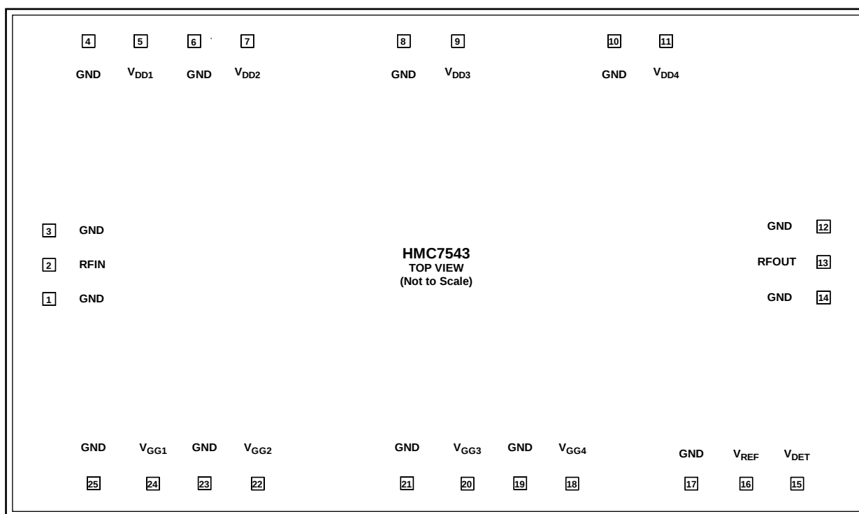
Figure 2. Pad Configuration
