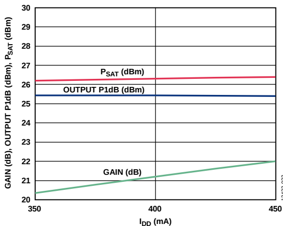
Figure 23. Gain, Output P1dB, and P_{SAT} vs. Drain Current ( I_{DD} ), RF = 71 GHz
