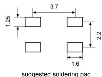
suggested soldering pad
