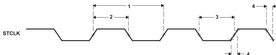
Figure 6-32. STCLK Timing
