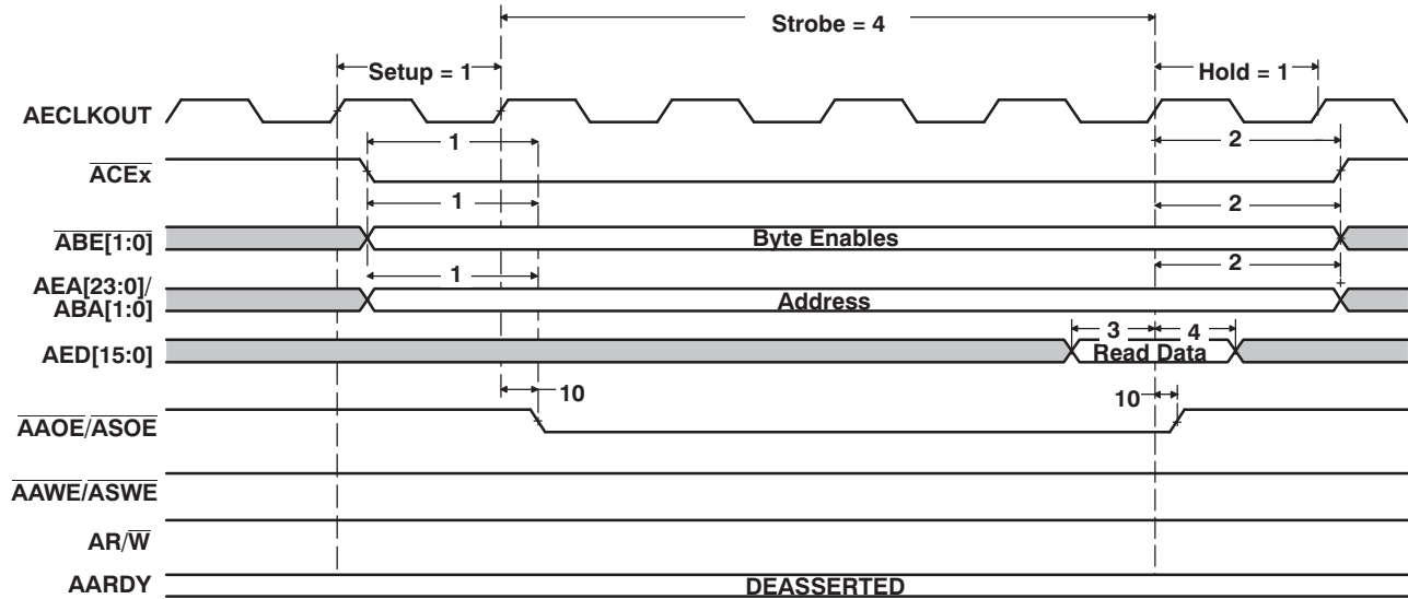
Figure 6-24. Programmable Synchronous Interface Read Timing for EMIFA (With Read Latency = 2)
