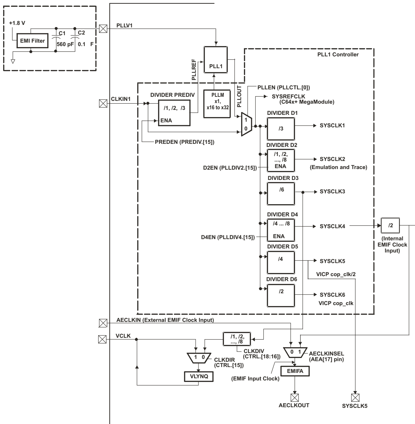
Figure 6-5. PLL Input Clock
