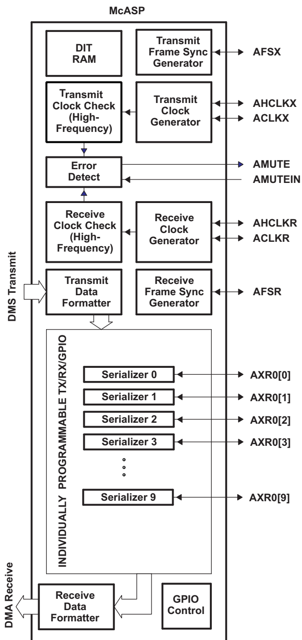
Figure 6-48. McASP Configuration
