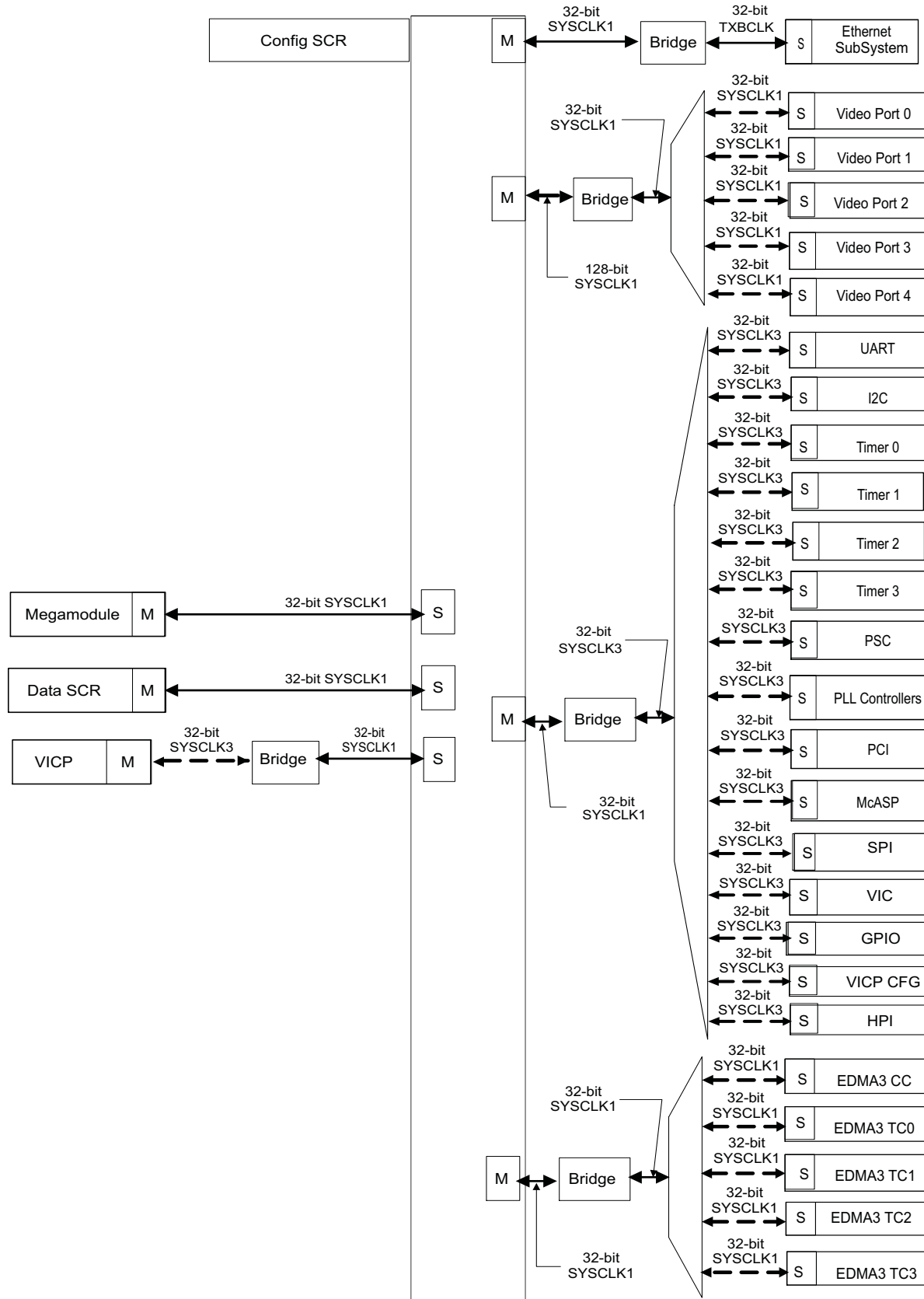
Figure 4-2. Configuration SCR
