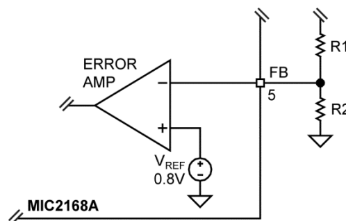
Figure 2. Voltage-Divider Configuration
