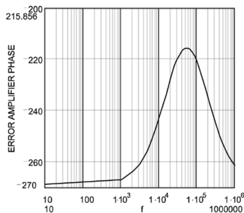
Figure 8. Error Amplifier Phase Curve
