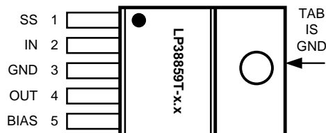
Figure 2. 5-Lead TO-220, Top View See NDH005D Package
