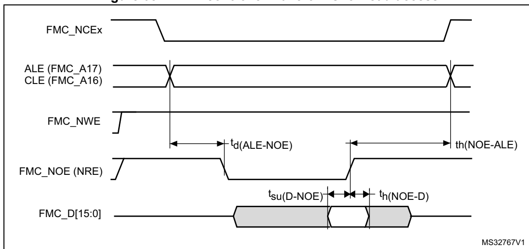
Figure 68. NAND controller waveforms for read access
