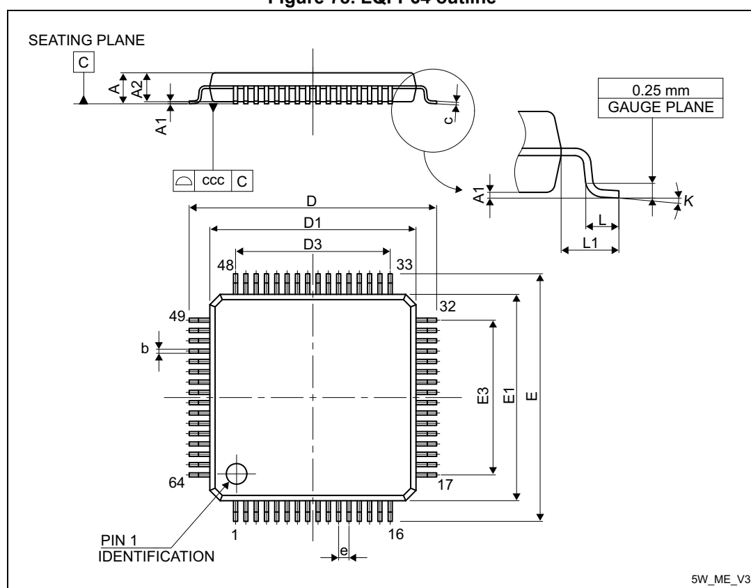
Figure 78. LQFP64 outline
