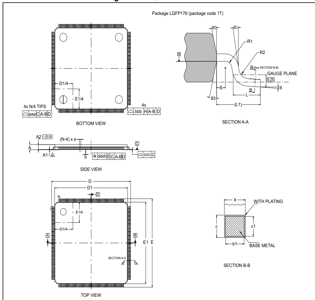
Figure 87. LQFP176 - Outline
