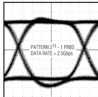
ELECTRICAL EYE DIAGRAM ( I_{\text{MODQ}} = 30\text{mA} )
