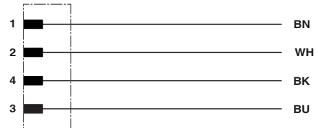
Contact assignment of the M8 plug
