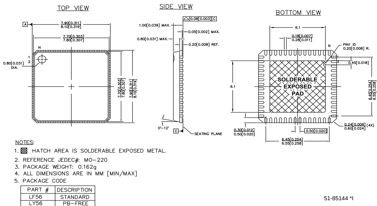
Figure 7. 56-pin QFN 8 \times 8 mm LF56A (Subcon Punch Type with 6.1 \times 6.1 EPad)
