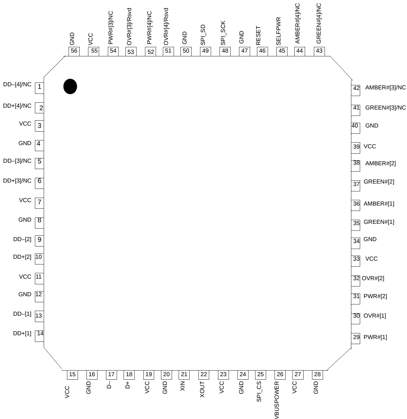
Figure 1. 56-pin Quad Flat Pack No Leads (8 mm × 8 mm) [2]
