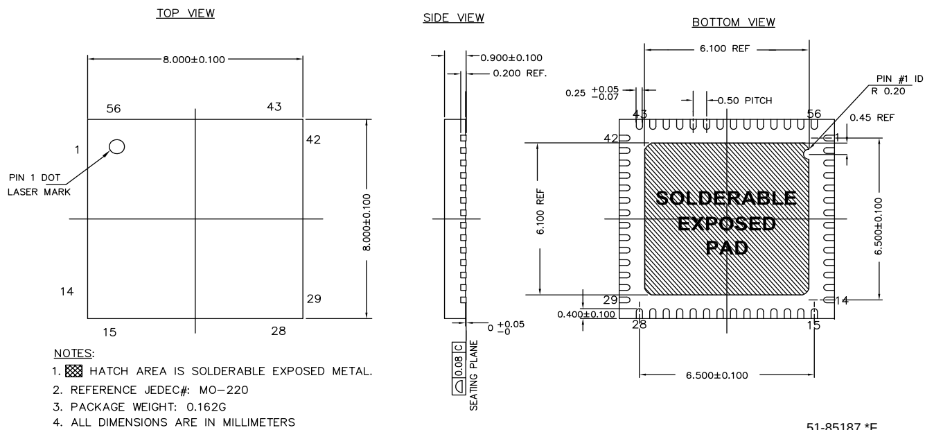
Figure 6. 56-pin Sawn QFN ( 8 \times 8 \times 1.00 mm)
