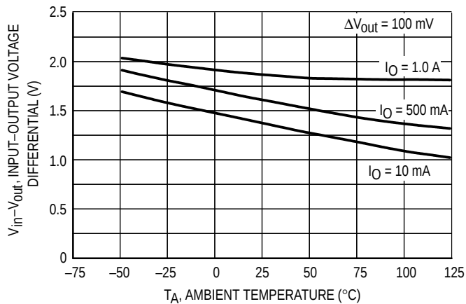
Figure 9. Dropout Voltage
