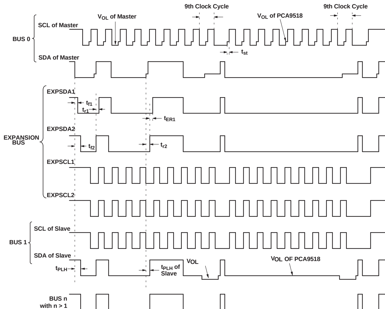
Figure 4. Bus Waveforms
