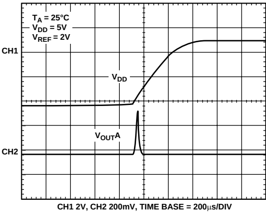
Figure 30. Power-On Reset to 0 V
