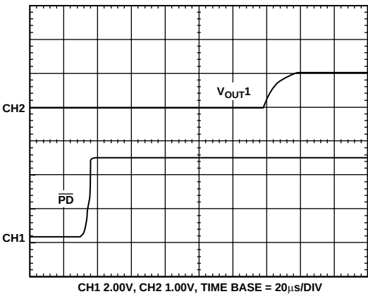
Figure 31. Exiting Power-Down to Midscale
