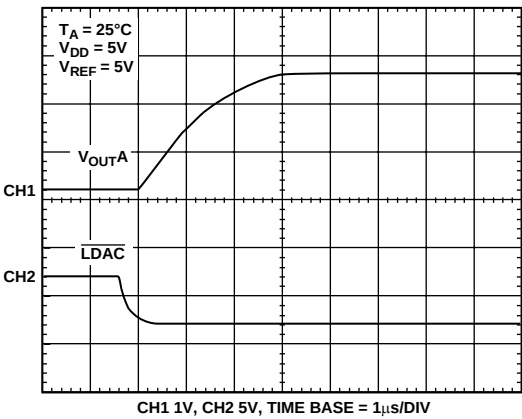
Figure 29. Half-Scale Settling (1/4 to 3/4 Scale Code)
