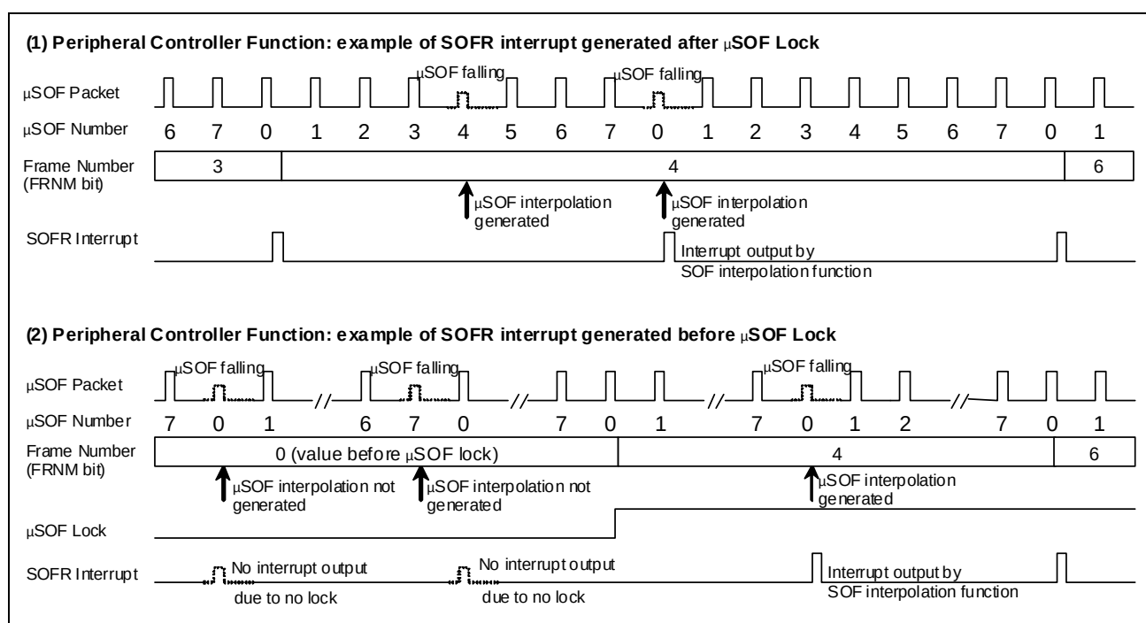
Figure 3.12 SOFR Interrupt Output Timing Example
