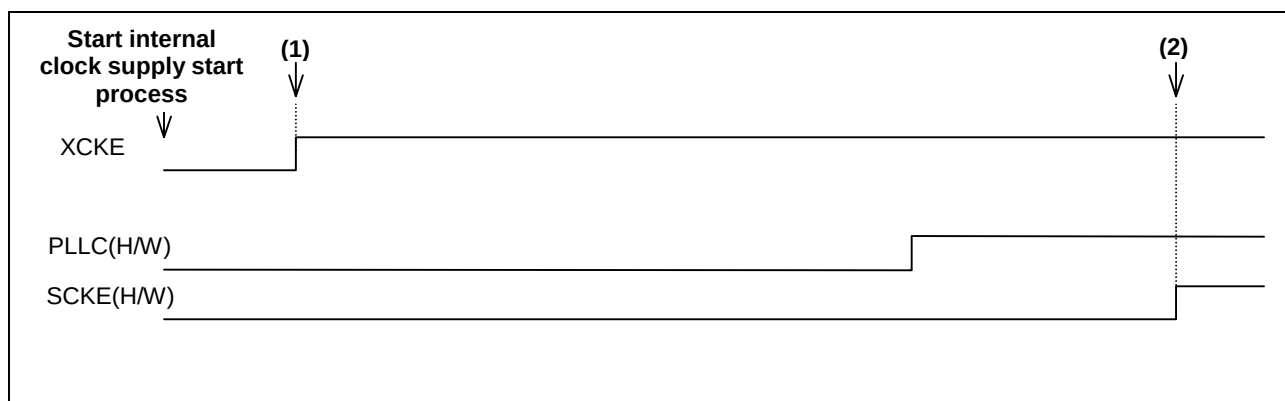
Figure 3.2 Clock Supply Start Control Timing Diagram
