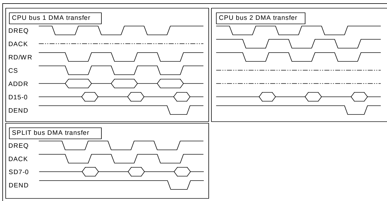
Figure 3.16 FIFO Port Access and DMA Control Pin
