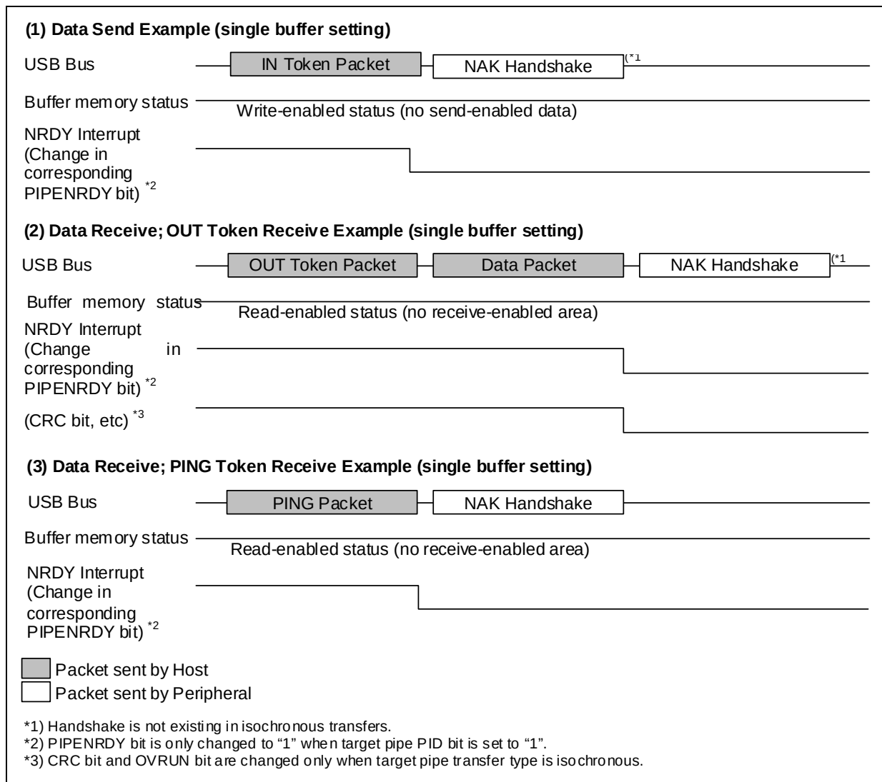
Figure 3.8 NRDY Interrupt Generation Timing for Peripheral Controller Function
