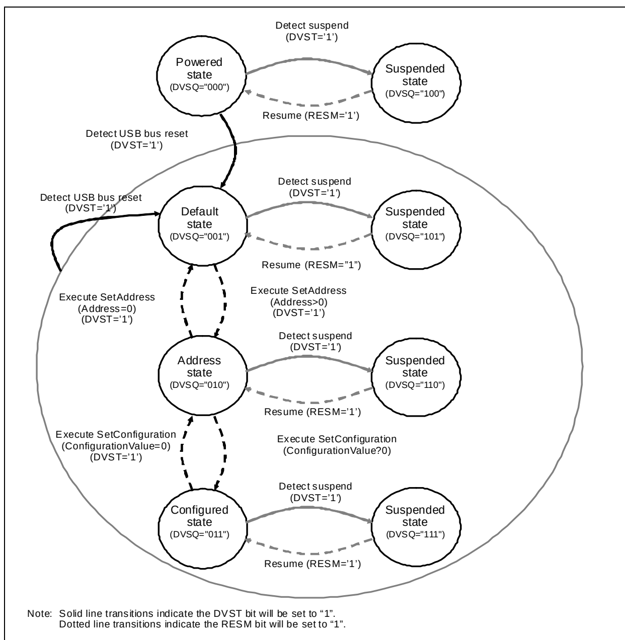
Figure 3.10 Device State Transitions
