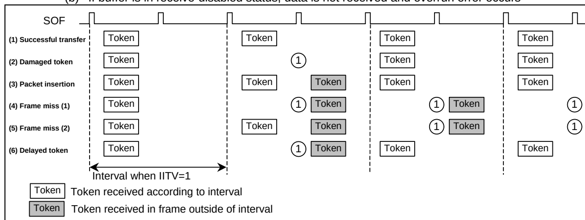
Figure 3.22 Interval Error Occurrence Example When "IITV=1"
