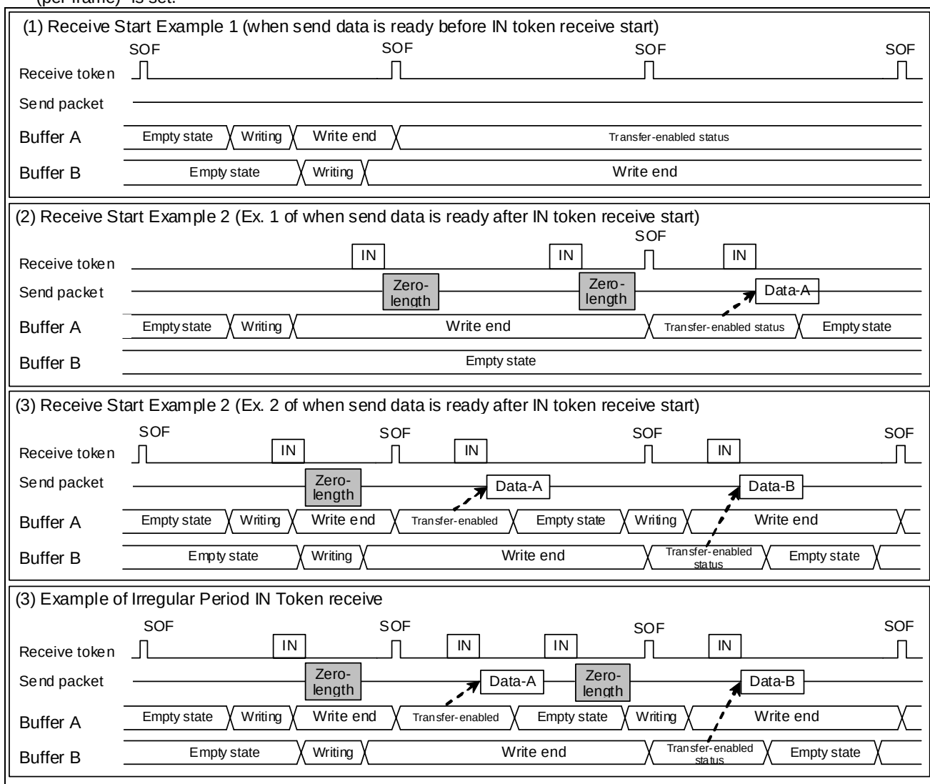
Figure 3.20 Data Setup Function Operation
