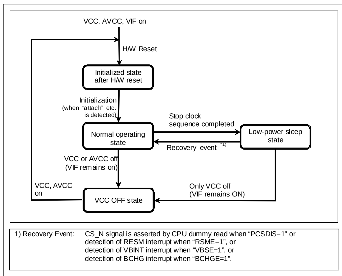
Figure 3.1 Controller State Transition Diagram
