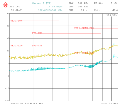
Figure 9-35. Conducted EMI versus CISPR25 Limits (Yellow: Peak Signal, Blue: Average Signal)
