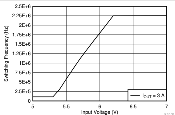
V_{OUT} = 5\text{ V} F_{SW} = 2100\text{ kHz} AUTO Mode Figure 9-24. LM61435-Q1 Frequency Dropout Curve
