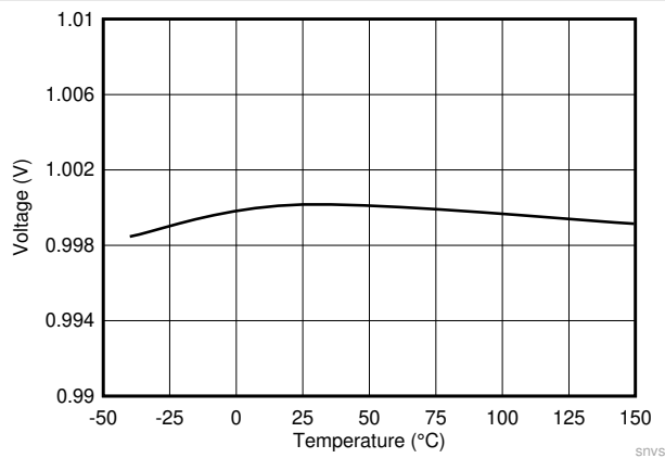
Figure 7-3. Feedback Voltage
