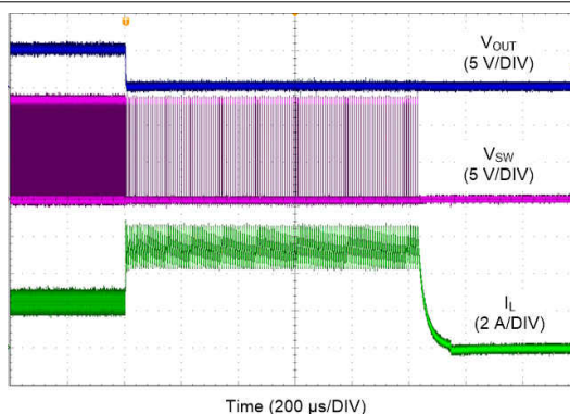
V_{OUT} = 5\text{ V} F_{SW} = 2100\text{ kHz} FPWM Mode I_{OUT} = 2.5\text{ A to Short Circuit} V_{IN} = 13.5\text{ V}
