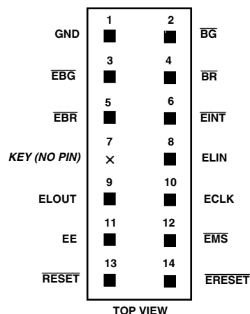
Figure 10. Target Board Connector for EZ-ICE
