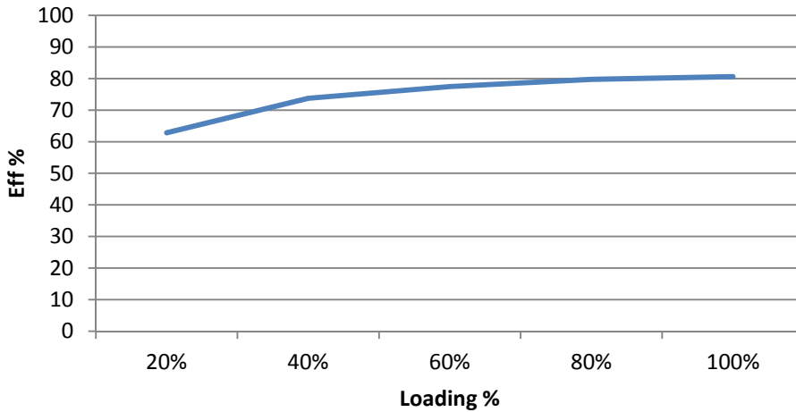
AM3G-2403SZ Efficiency vs. Loading
