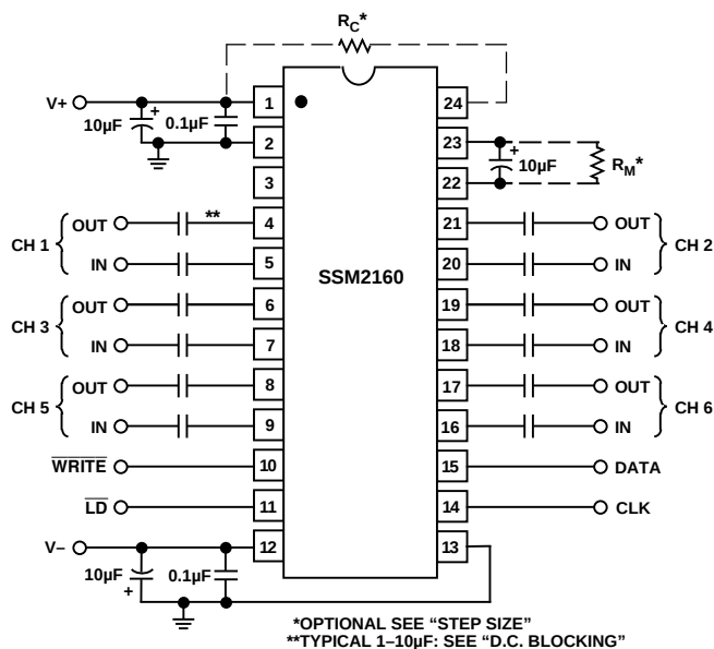
Figure 25. Typical Application Circuit (Dual Supply)
