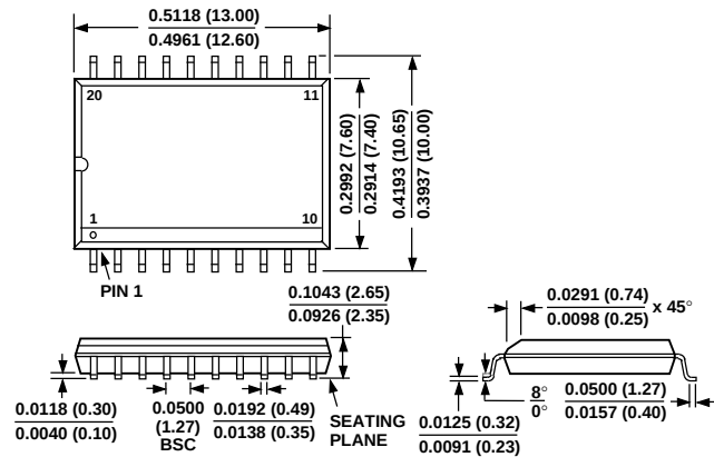
20-Lead SOL (R-20)
