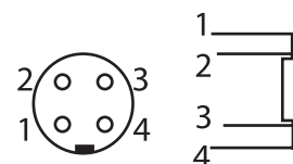
4-wire Pt100
