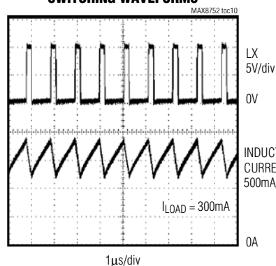
SWITCHING WAVEFORMS
