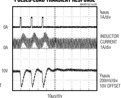
PULSED-LOAD TRANSIENT RESPONSE
