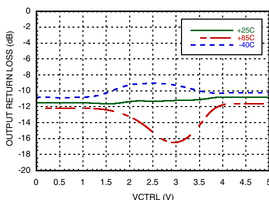
Output Return Loss vs. VCTRL
