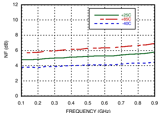
Noise Figure vs. Frequency over Temperature [1] [3]
