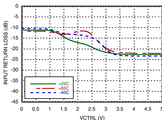
Input Return Loss vs. VCTRL @ 800MHz [2]
