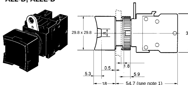
Square Full-guard Type A22-D, A22L-D
