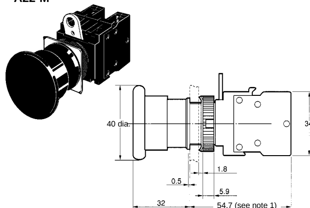
40-dia. Mushroom Type A22-M
