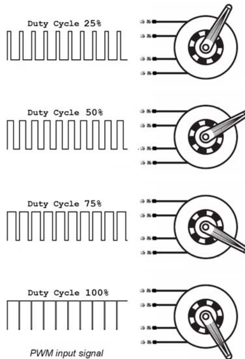
Figure 6. Stepper Motor Gauges at Different Duty Cycles
