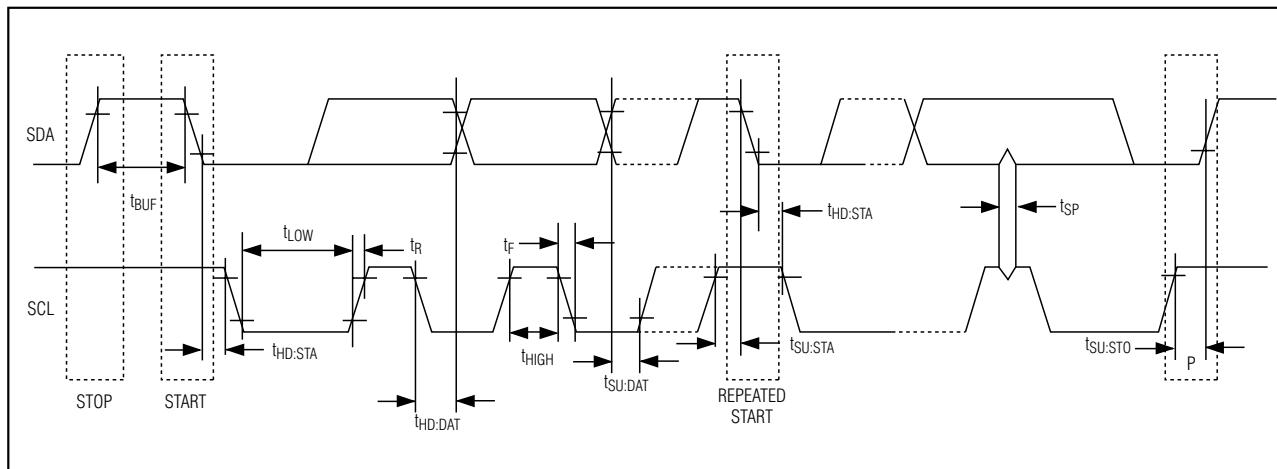
Figure 1. I²C Serial Interface Timing Diagram
