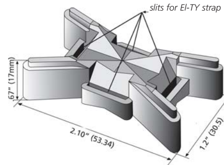
El-Ty Spacer
