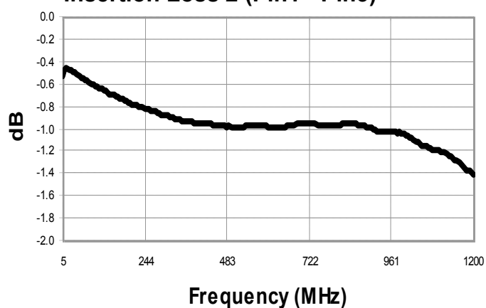
Insertion Loss 2 (Pin1 - Pin3)
