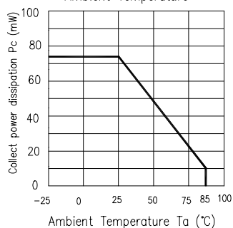
Fig.1 Collector Power Dissipation vs. Ambient Temperature
