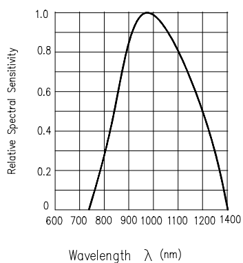
Fig.5 Spectral Sensitivity
