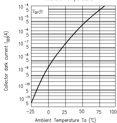
Fig.2 Collector Dark Current vs. Ambient Temperature
