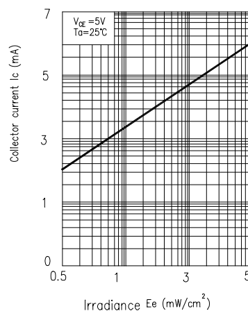
Fig.4 Collector Current vs. Irradiance
