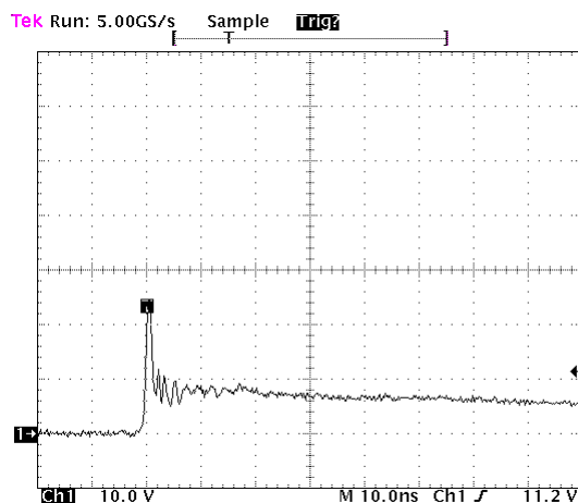
ESD Response (8kV Contact per IEC 61000-4-2)
