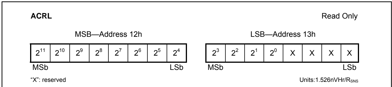
Figure 9. Fractional/Low Accumulated Current Register Format, ACRL
