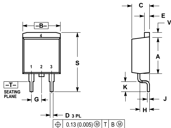
CASE 418B-03 ISSUE C
