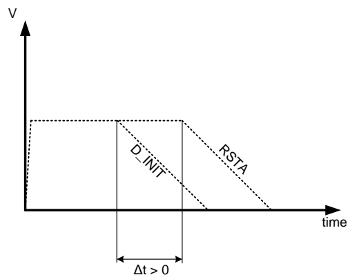
Figure 13-6. D_INIT & RSTA realease sequence during power-on
