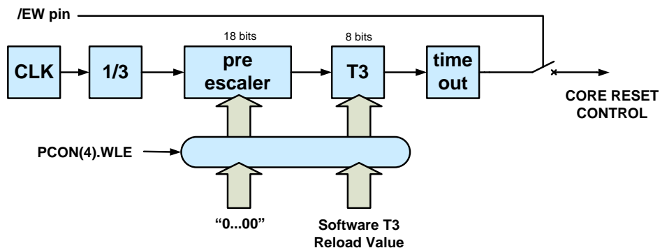
Figure 5-4. Watchdog timer
