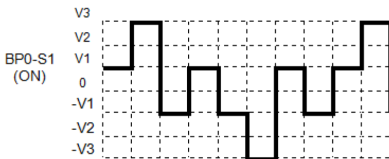
Figure 10-8. BP0-S1 segment 1/4 duty voltage waveform
