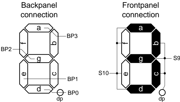
Figure 10-9. Example LCD 7-segment connections
