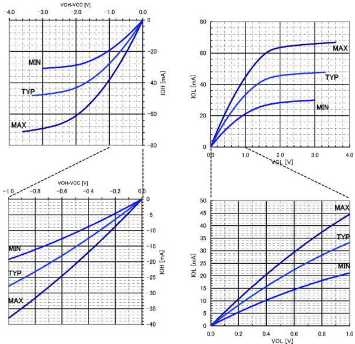
Figure 13-1. CMOS IO L and M type,V-I curves
