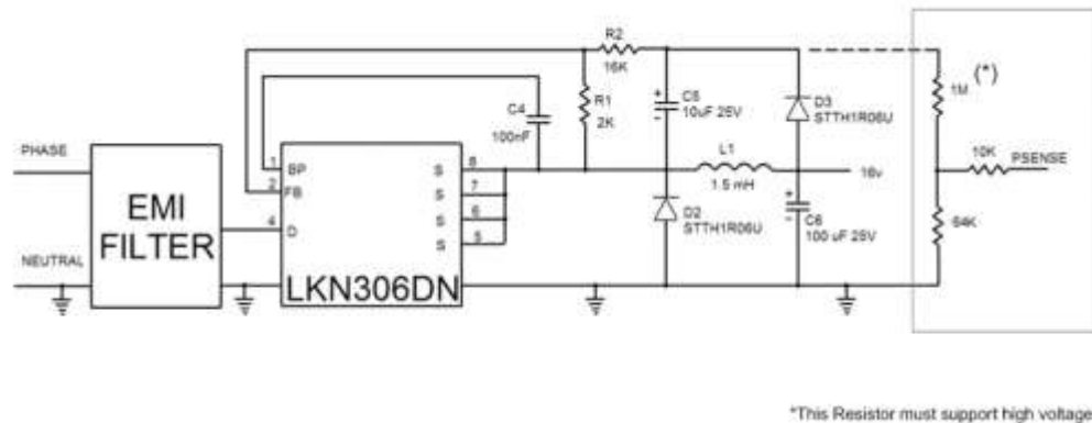
Figure 12-7. PSENSE application circuit
