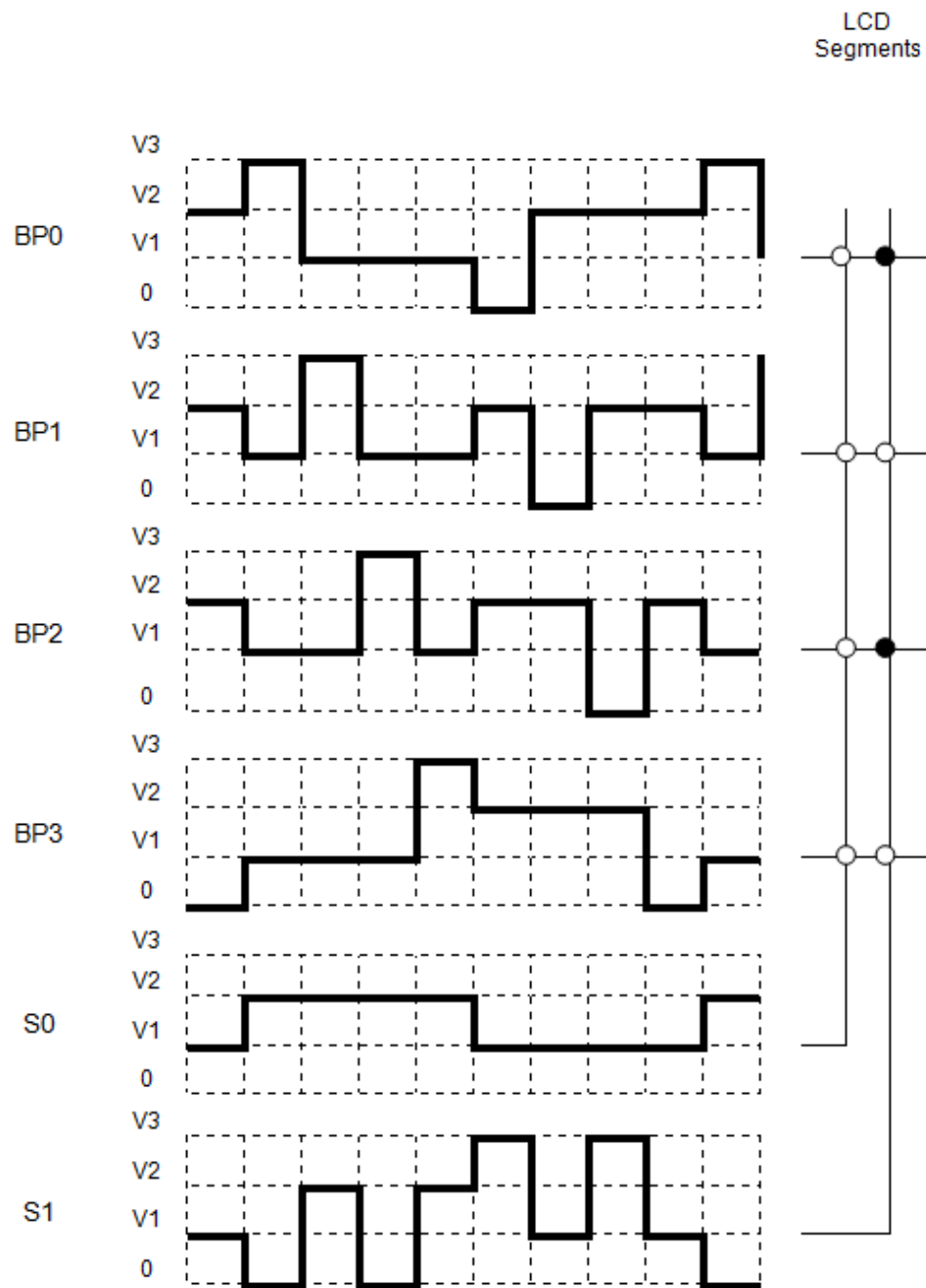
Figure 10-6. LCD ¼ duty waveforms
