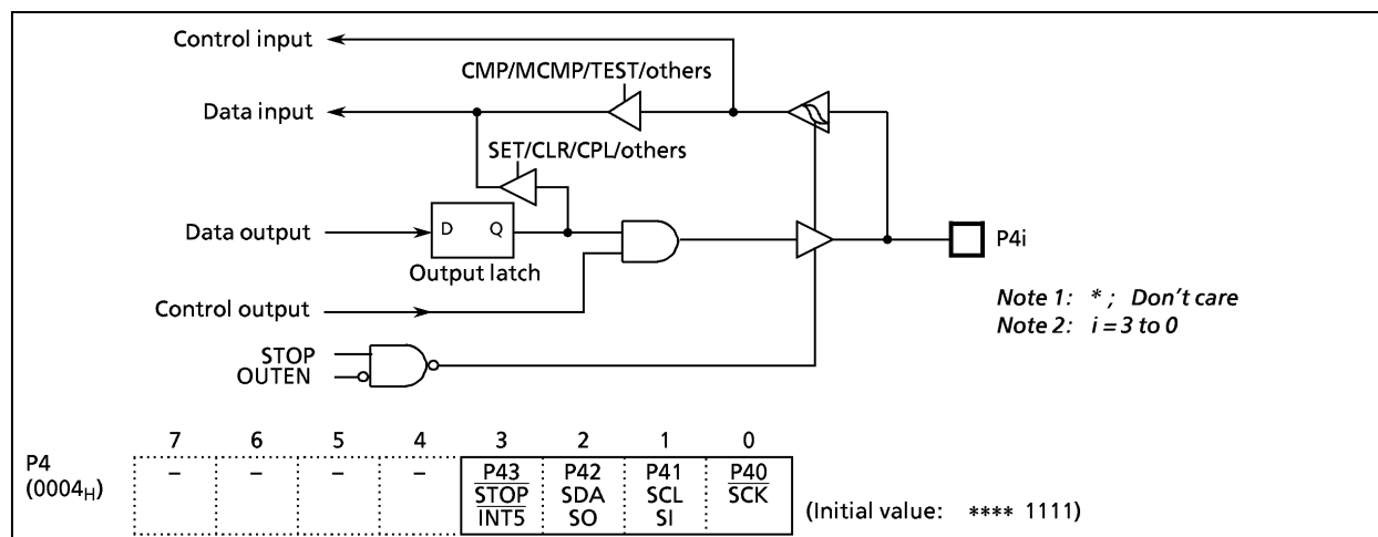
Figure 2-4. Port P4
