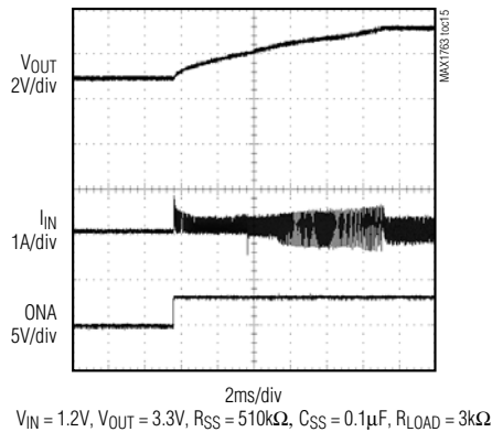
STARTUP WAVEFORMS USING SOFT-START
