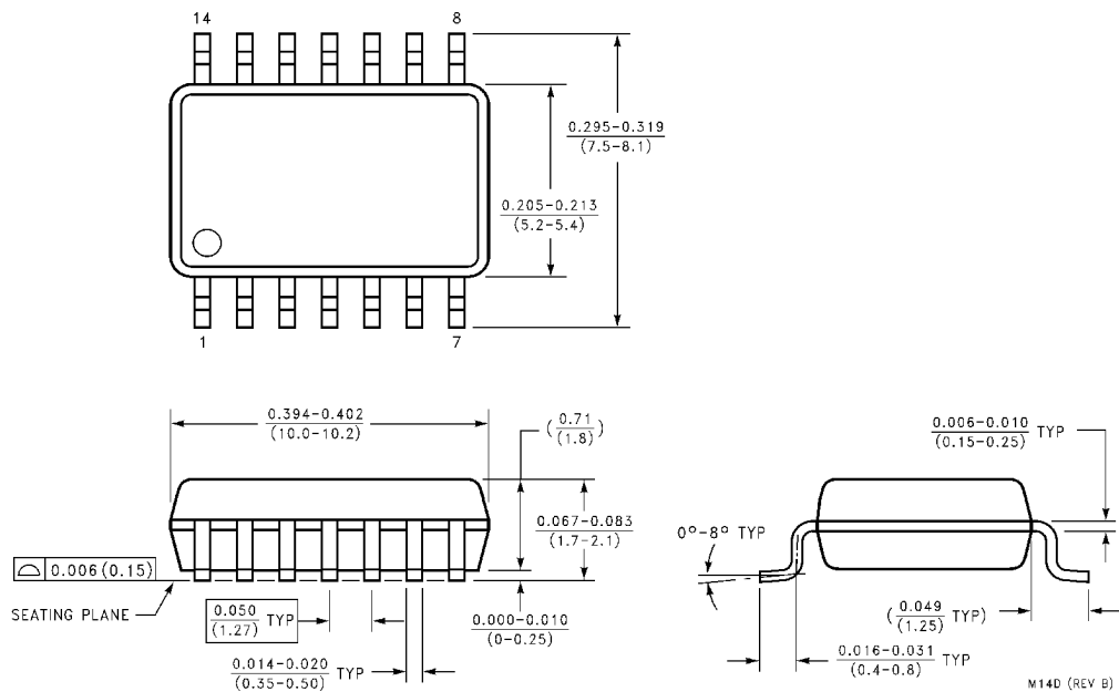
Small Outline Package (SJ) Order Number DM74ALS02SJ Package Number M14D
