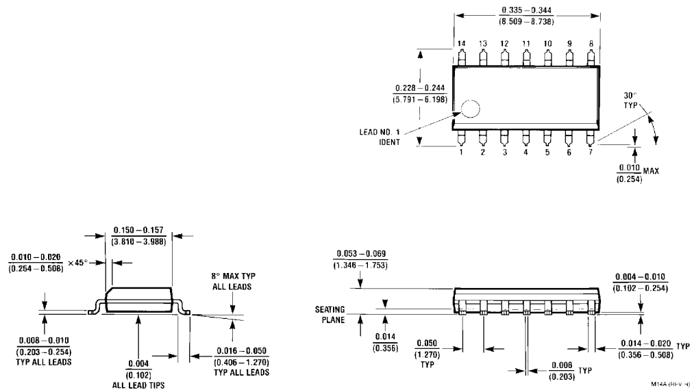
S.O. Package (M) Order Number DM74ALS02M Package Number M14A
