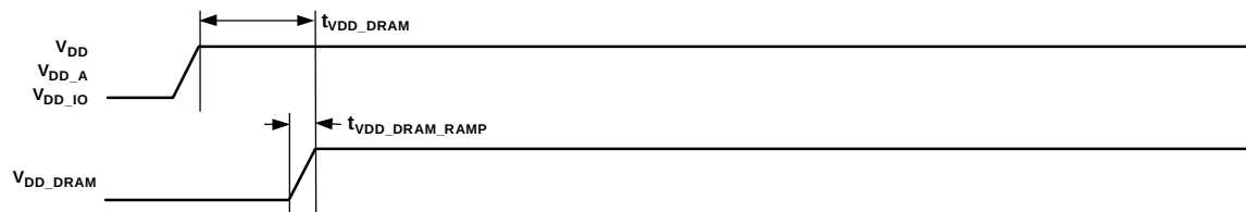
Figure 8. Power-Up Timing
