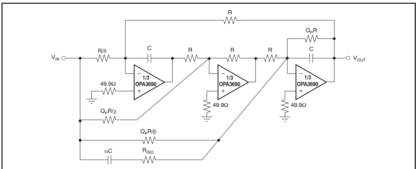
Figure 46. State Variable Filter
