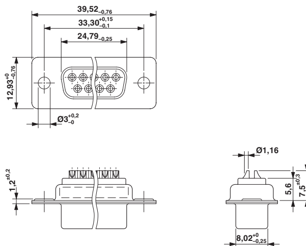
Dimensional drawing
