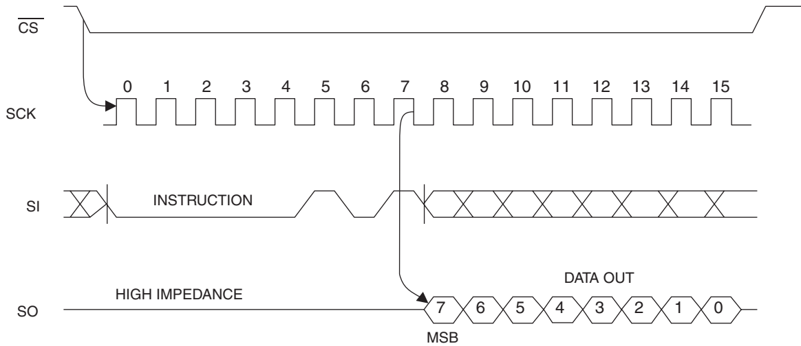
Figure 6. RDSR Timing
