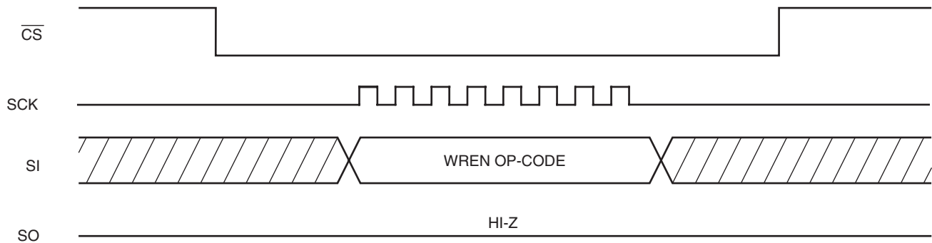
Figure 4. WREN Timing
