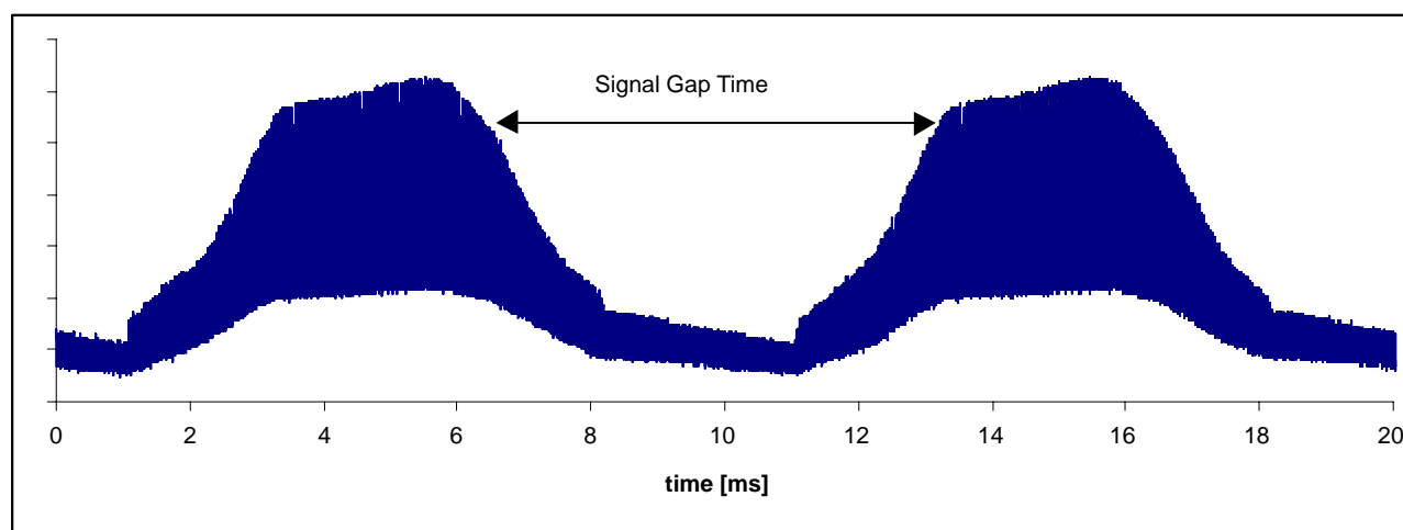
Figure B: Disturbance Signal from Fluorescent Lamp with Signal Gap Time of 7ms (suppressed by TSOP18..SS3V)
