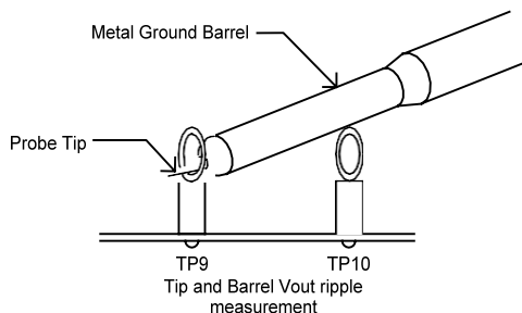
Figure 4-2. Output Ripple Measurement – Tip and Barrel Using TP9 and TP10
