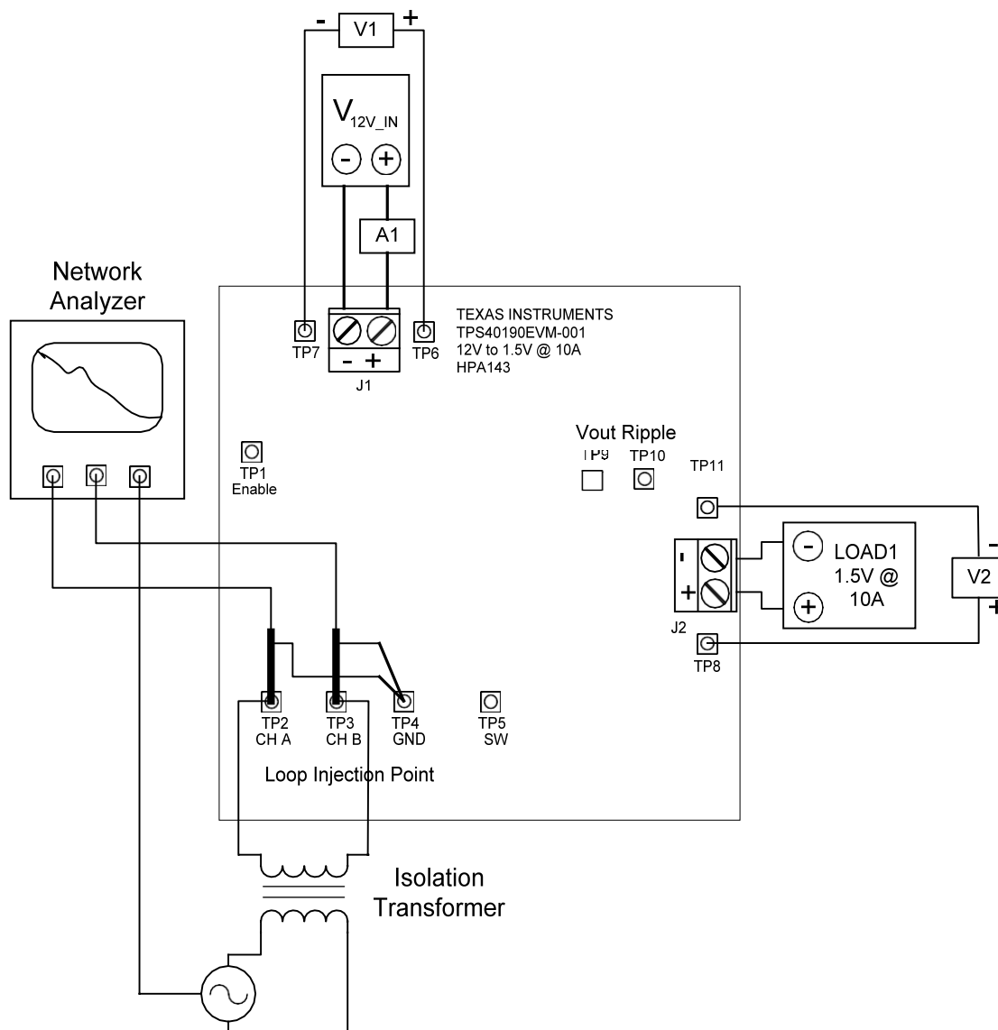
Figure 4-3. Control Loop Measurement Setup
