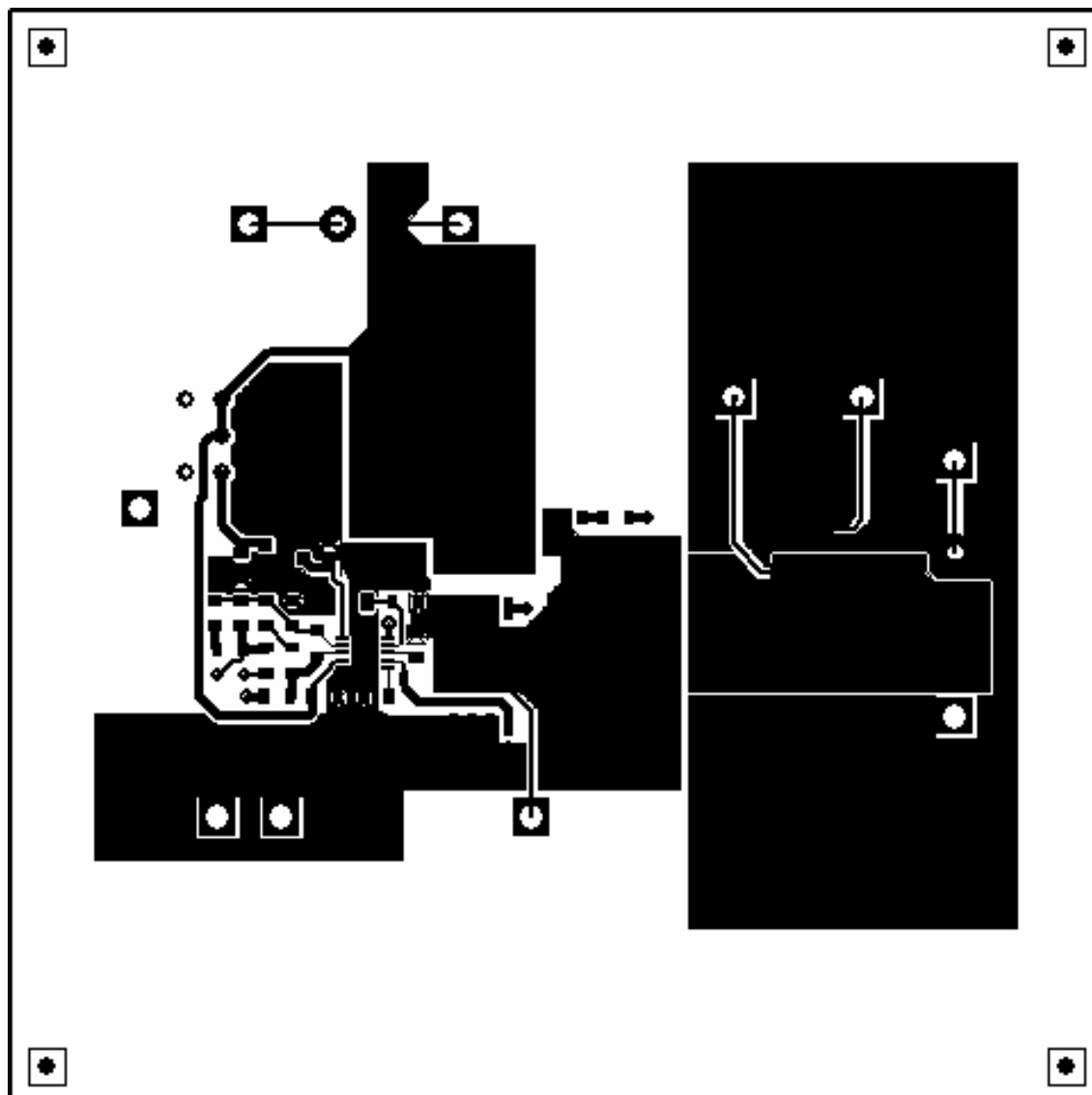
Figure 6-3. TPS40190EVM-001 Top Copper (Viewed from Top)
