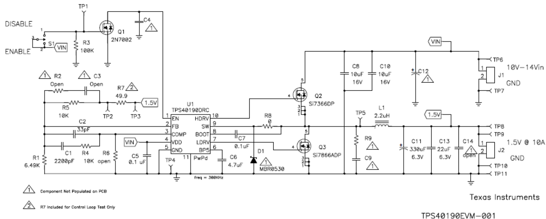
Figure 3-1. TPS40190EVM-001 Power Stage/Control Schematic
