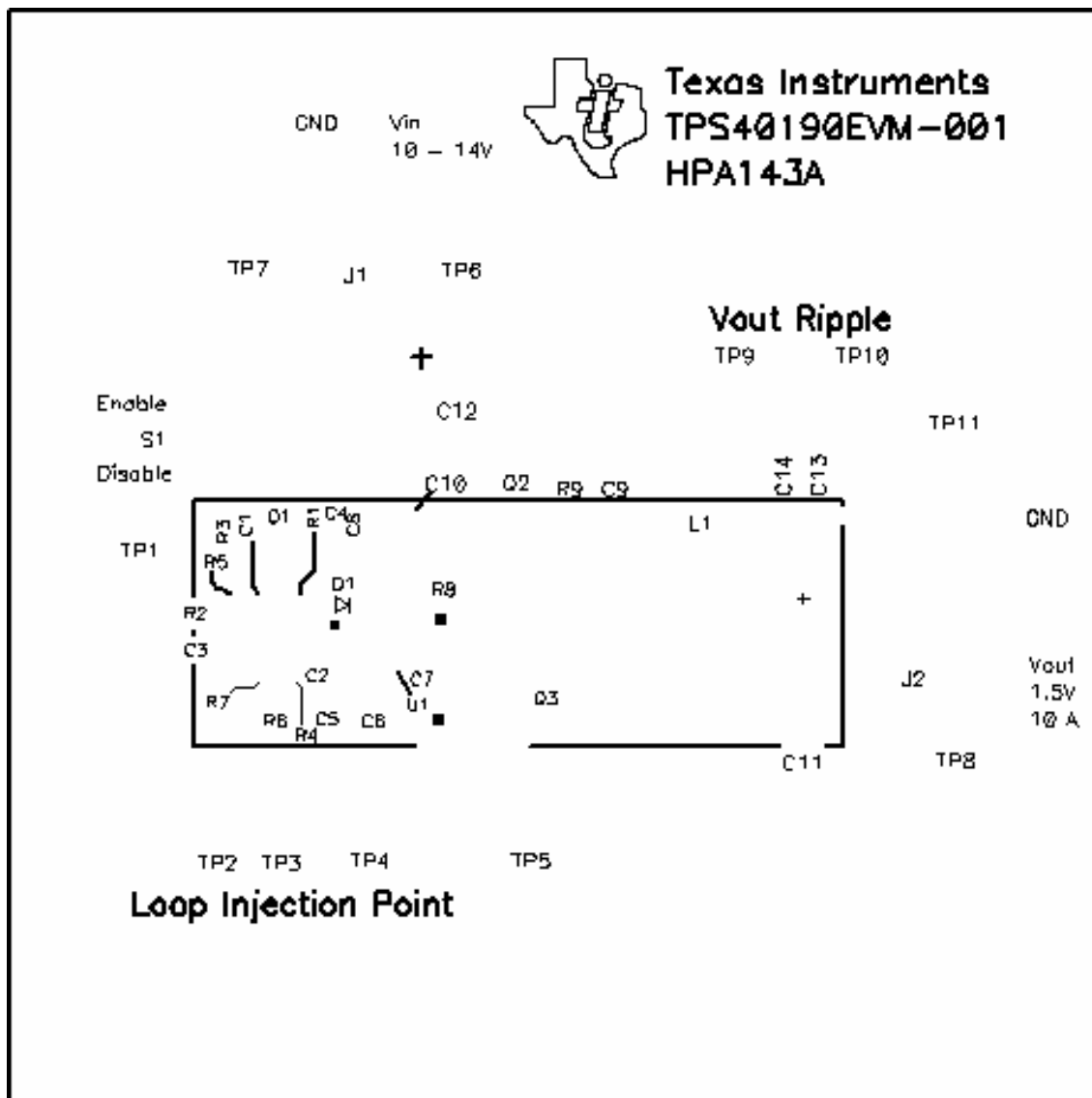
Figure 6-2. TPS40190EVM-001 Silkscreen (Viewed from Top)
