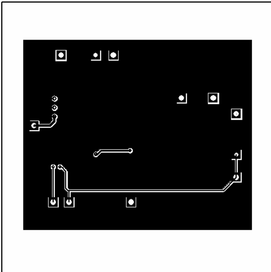
Figure 6-4. TPS40190EVM-001 Bottom Copper (X-Ray View from Top)
