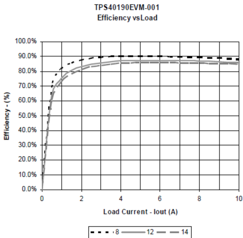
Figure 5-1. TPS40190EVM-001 Efficiency, V_{IN} = 10\text{ V to }14\text{ V} , V_{OUT} = 1.5\text{ V} , I_{OUT} = 0\text{ A to }10\text{ A}
