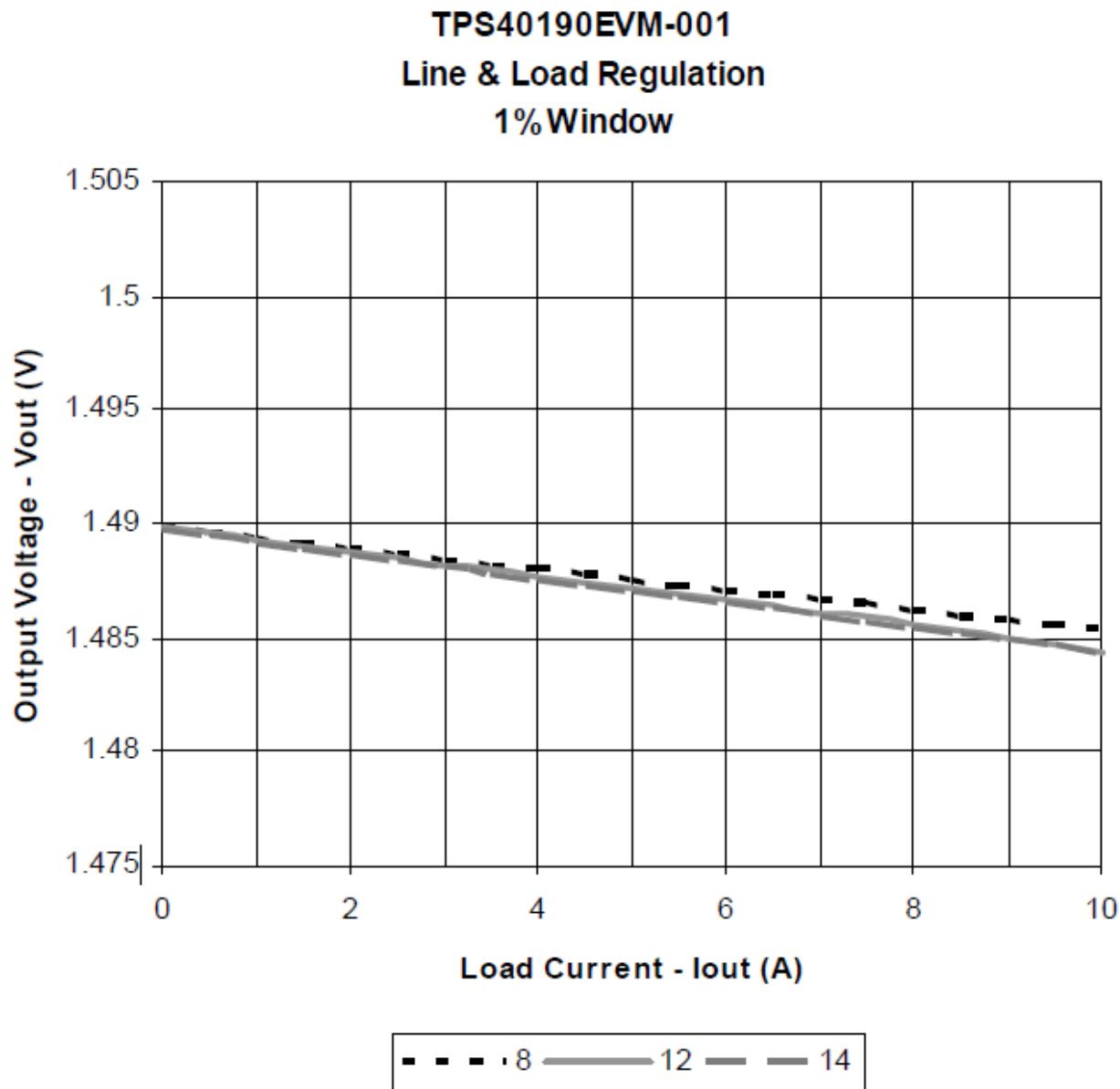
Figure 5-2. TPS40190EVM-001 Line and Load Regulation
