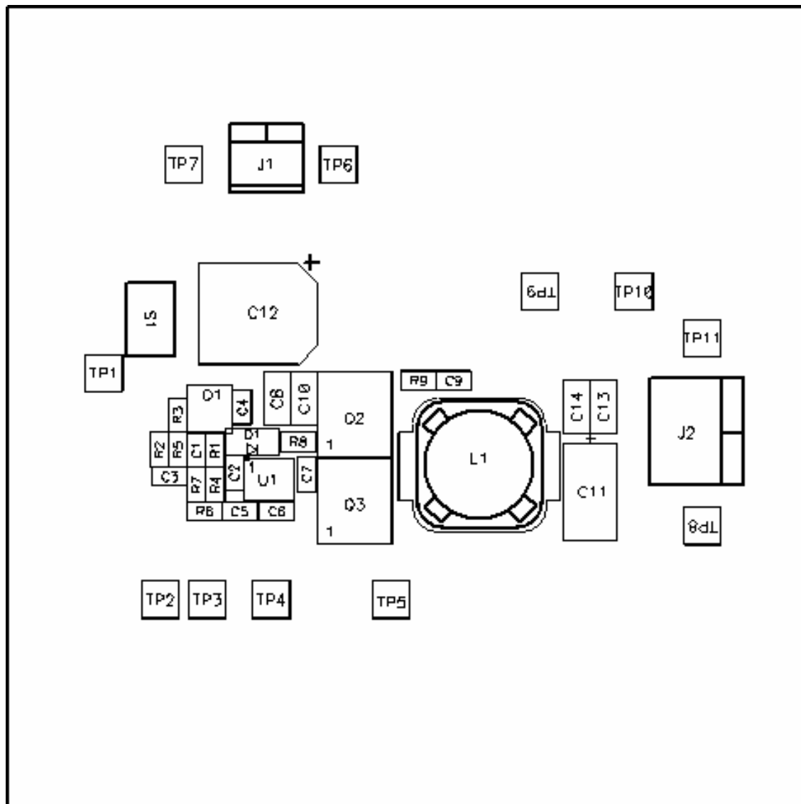
Figure 6-1. TPS40190EVM-001 Component Placement (Viewed from Top)
