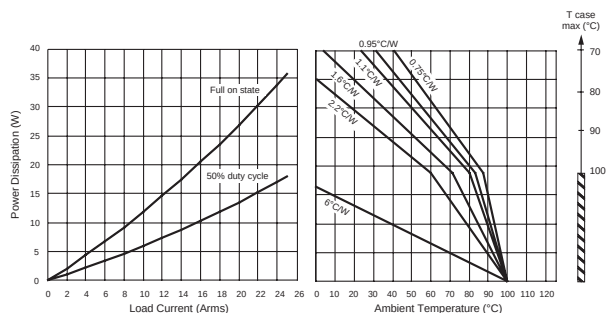
Figure 5b — 25A output current
