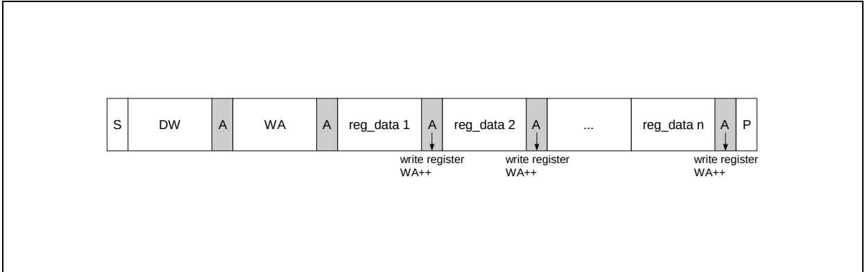
Figure 22. Page Write
