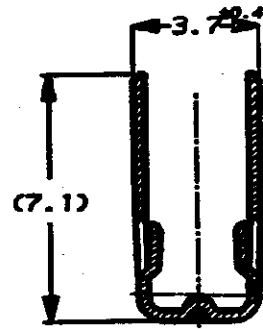
SECT B-B
