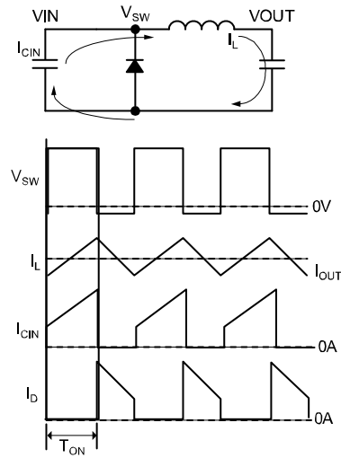
Figure 3. On-Time
