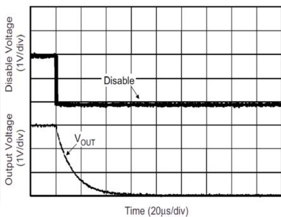
Figure 23. Shutdown Delay
