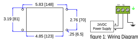
figure 1: Wiring Diagram
