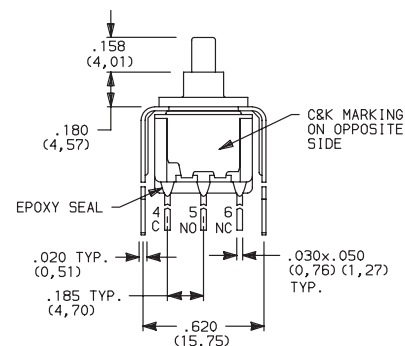
8221SD3_GE DPDT
